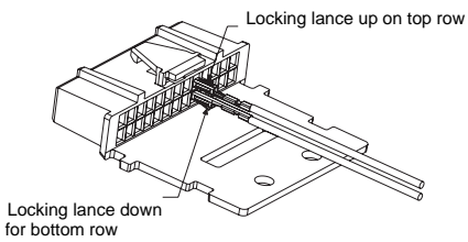
Figure 2. Terminal Orientation
