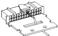
Figure 1a. Wire Strain Relief
