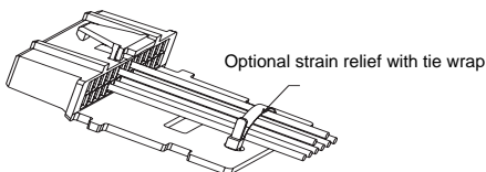
Figure 1b. Optional Strain Relief
